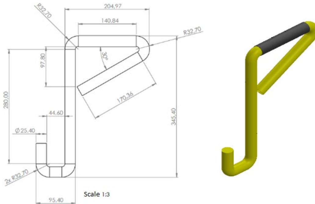
Figure 3: Tool specifications
